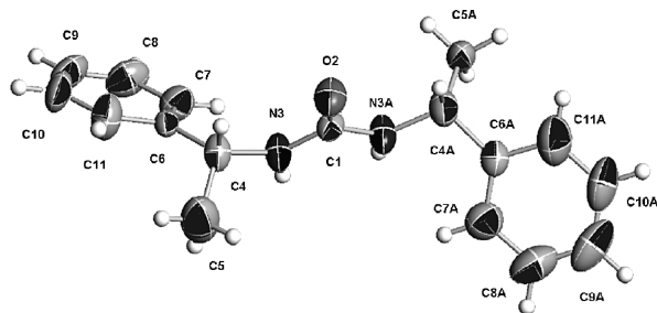
Figure 2. X-ray crystallographic structure and solid-state conformation of N,N' -bis[( R )-1-phenylethyl]urea, ( R,R )- 2
