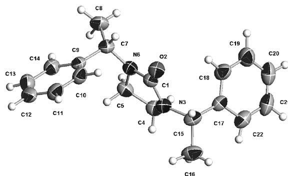
Figure 3. X-ray crystallographic structure and solid-state conformation of N,N' -bis[( S )-1-phenylethyl]ethyleneurea, ( S,S )- 3
