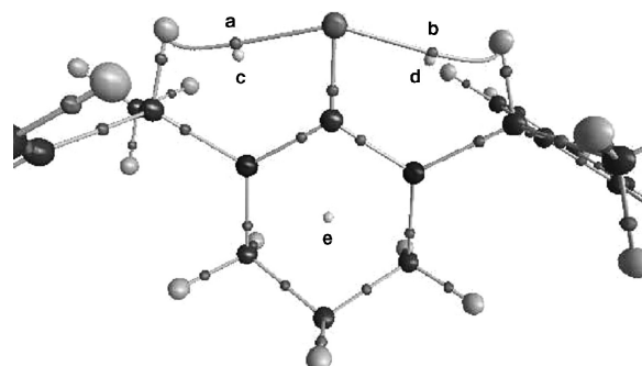
Figure 1. Critical points and bonding trajectories in the electron density of ( R,R )- 1 calculated at the HF/6-311+G**/HF/6-31G** level of theory (for clarity, Ph groups have been deleted)
