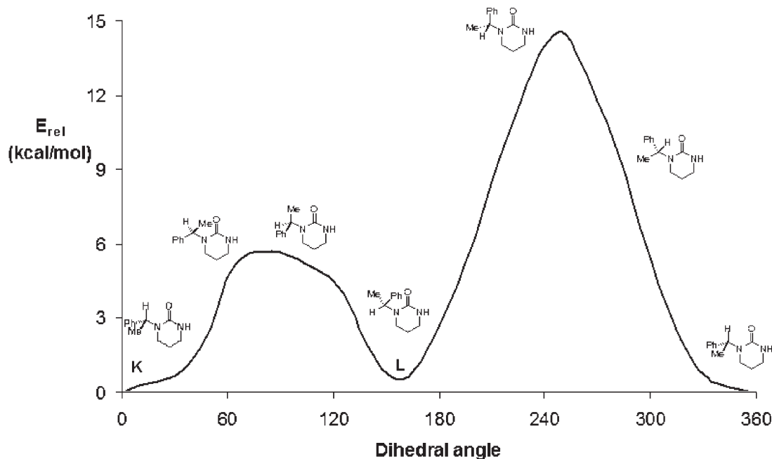
Figure 4. Rotation around the N—C* bond in ( R )- 6 , according to HF/3–21G* calculations (fully optimized geometries)
